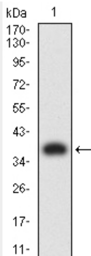
Figure 2: Western blot analysis using CD183 mAb against human CD183 (AA: extra mix) recombinant protein. (Expected MW is 38.3 kDa)
