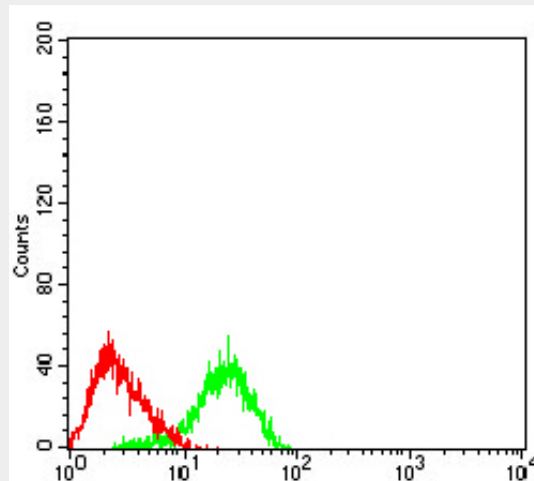
Figure 5: Flow cytometric analysis of Ramos cells using CD183 mouse mAb (green) and negative control (red).
